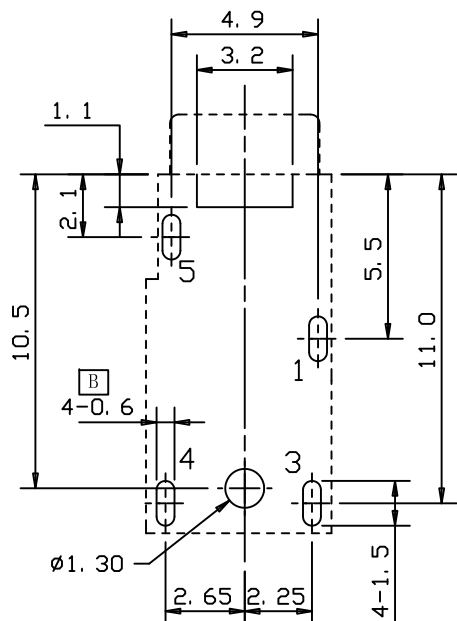
Recommended Pads Layout <BOTTOM VIEW>
