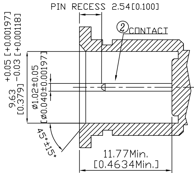
G PLUG DETAIL
