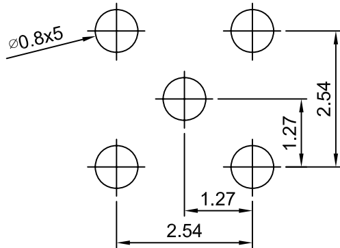
PCB Mounting Hole
