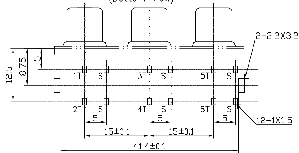
Dimensions of PC board holes(Commend) (Bottom View)
