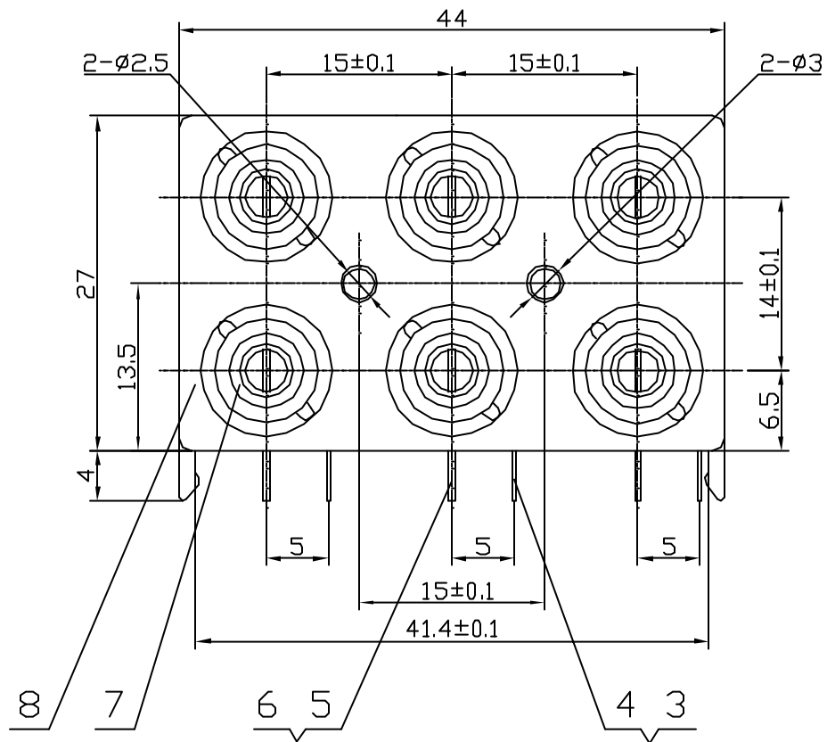
Dimensions of PC board holes(Commend) (Bottom View)
