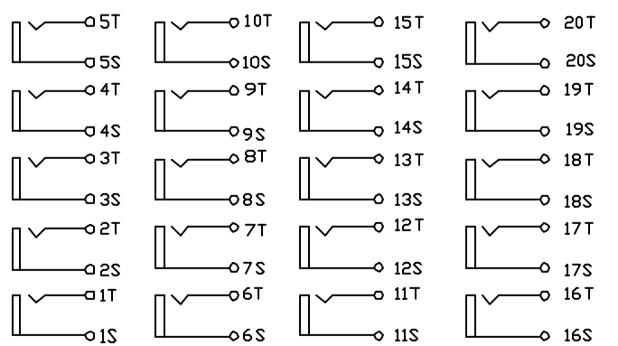
D CIRCUIT
