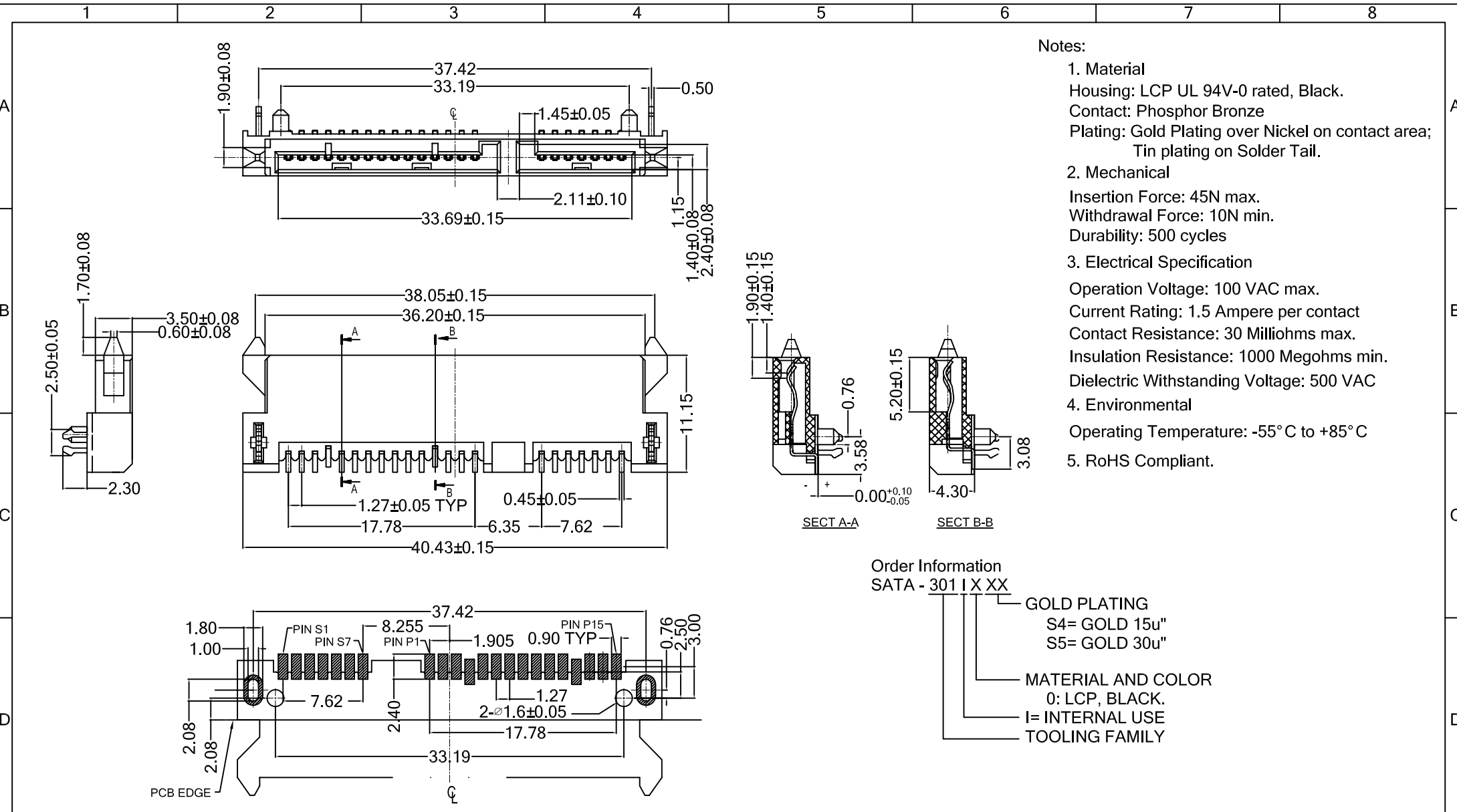
P.C.B LAYOUT (T=1.20) TOP VIEW
