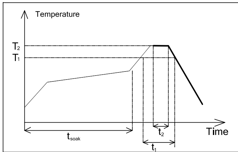
Figure 1. Reflow profile for solderability testing.
