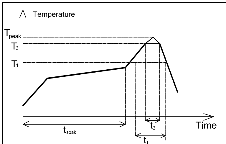
Figure 2. Reflow profile for soldering heat resistance testing
