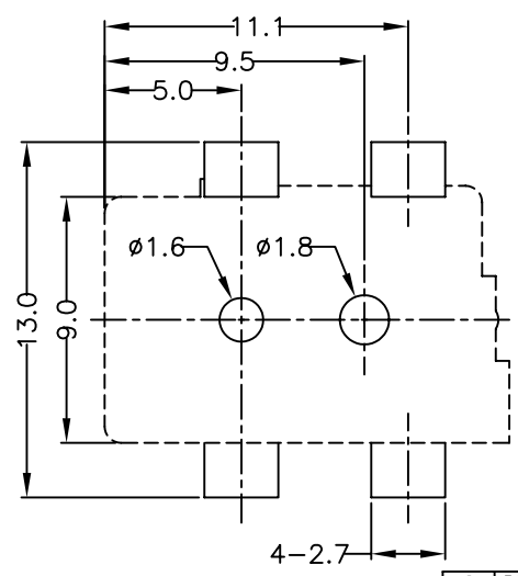
Recommended PAD Layout [TOP VIEW]
